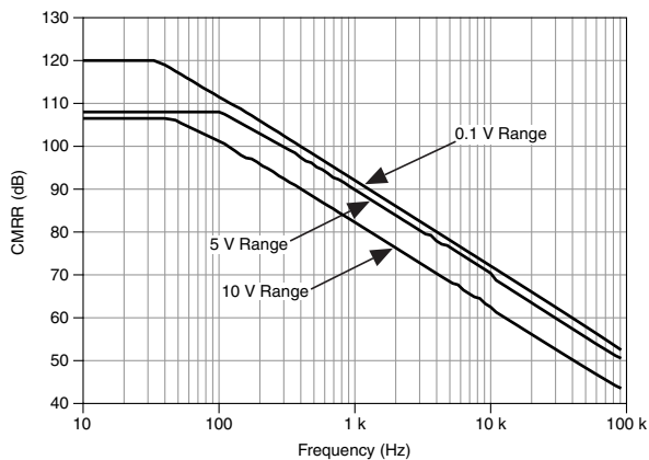
Figure 1. AI <0..31> CMRR
