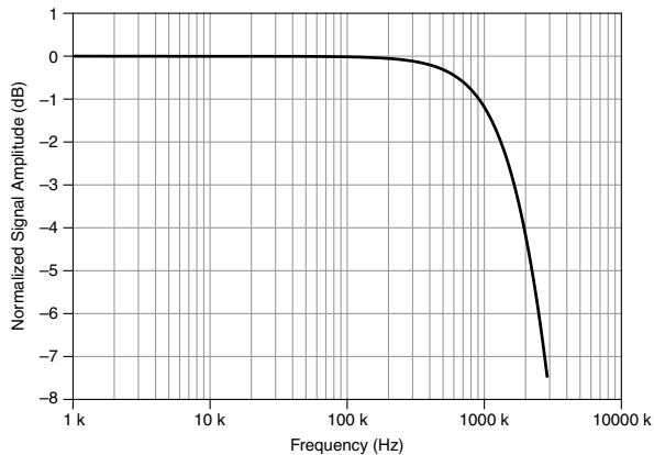
Figure 2. AI <0..31> Small Signal Bandwidth
