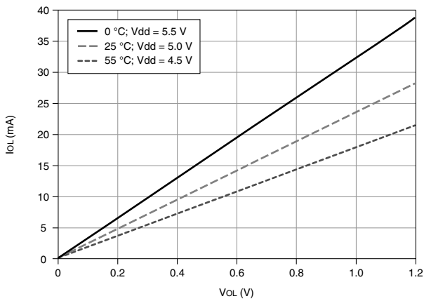
Figure 8. PFI <0..15>/P1/P2: I OL versus V OL
