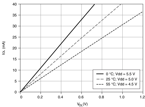
Figure 6. P0.<0..31>: I_{OL} versus V_{OL}
