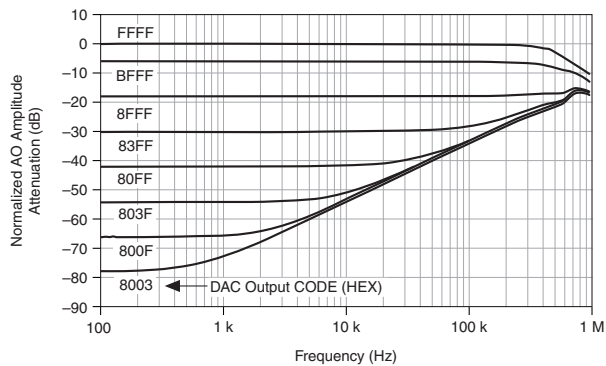
Figure 4. AO <0..3> External Reference Bandwidth
