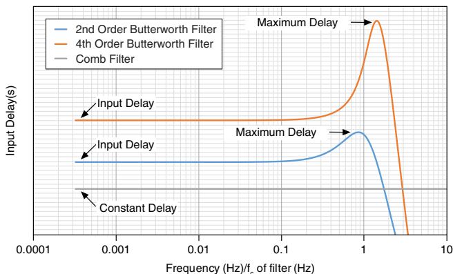
Figure 9. Comparing Typical Input Delay for NI 9253 Filters
