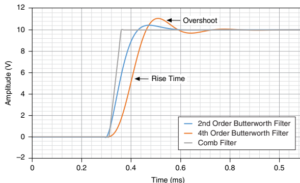
Figure 11. Comparing Typical Step Response of NI 9253 Filters
