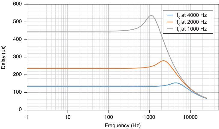
Figure 5. Butterworth Filter Input Delay (4th Order, with 12.8 MHz Timebase, 4000 Hz, 2000 Hz, 1000 Hz)
