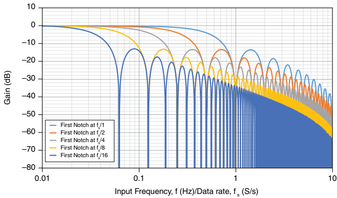
Figure 4. Typical Comb Filter Flatness
