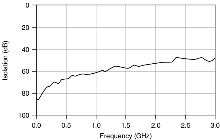
Figure 4. Isolation, Typical
