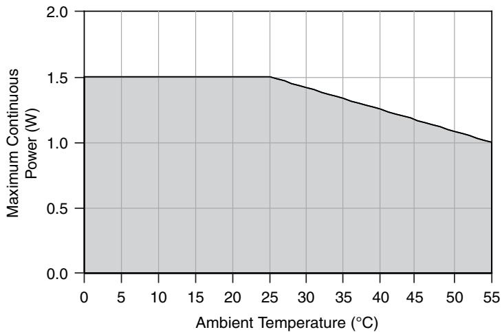
Figure 5. Termination Derating
