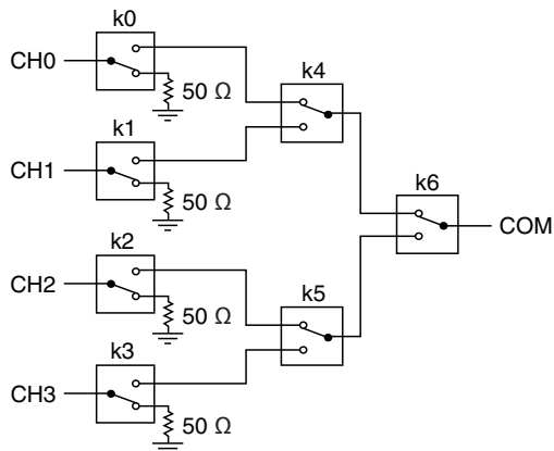
Figure 6. PXI-2545 Power-On State
