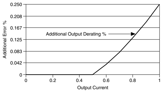
Figure 2. Accuracy Specification Derating versus Output Current
