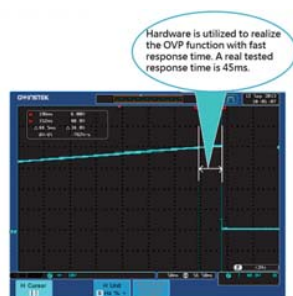
OVP Trigger
