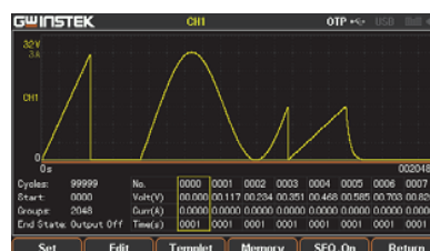
Output Waveform of the GPP-X323 Series
