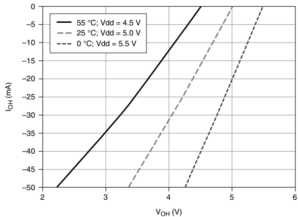
Figure 2. P0.<0..7>: I_{OH} versus V_{OH}
