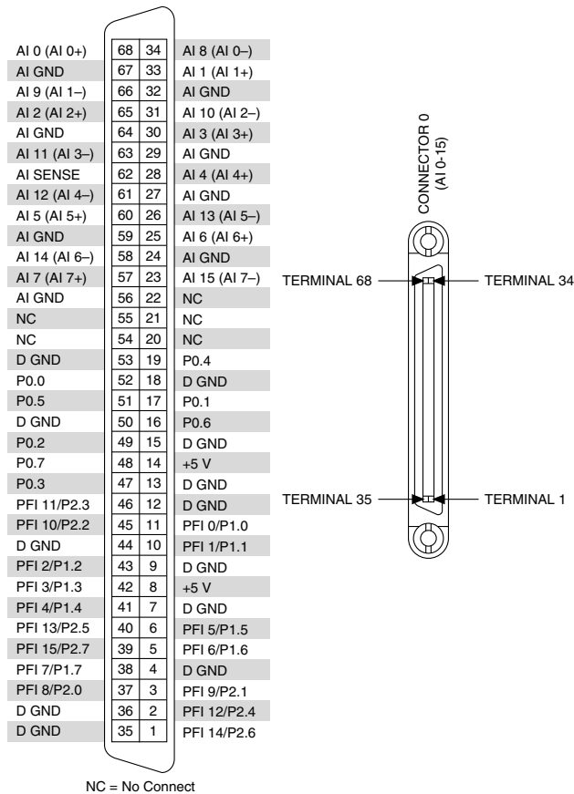
Figure 6. NI PCIe-6320 Pinout
