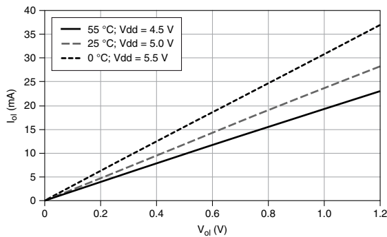
Figure 8. Digital I/O (PFI <0..15>/P1/P2): I ol versus V ol
