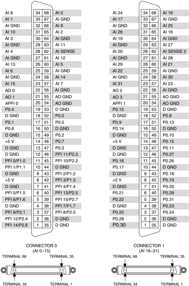
Figure 10. NI USB-6289 Mass Termination Pinout
