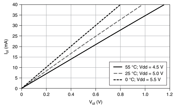
Figure 7. Digital I/O (P0.<0..31>): I ol versus V ol
