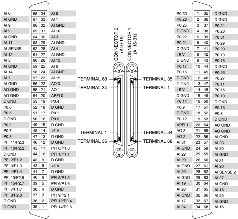
Figure 9. NI PCI/PXI-6289 Pinout
