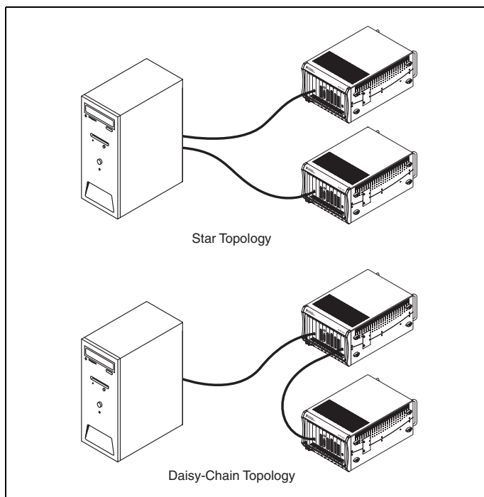
Figure 1-5. Example of MXI-Express Gen II x8 System Expansion Topologies
