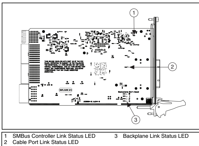
Figure 2-5. NI PXIe-8381 Back Side LED Locations
