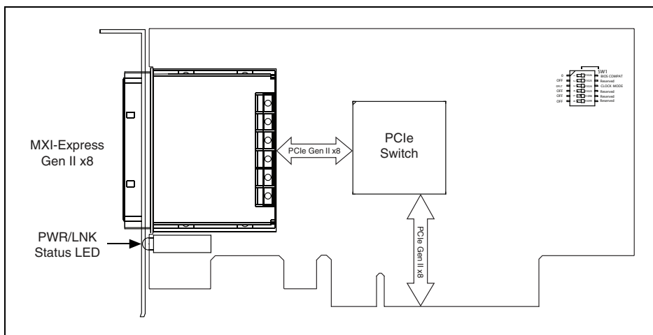
Figure 1-1. NI PCIe-8381 (153094x-01L) Block Diagram
