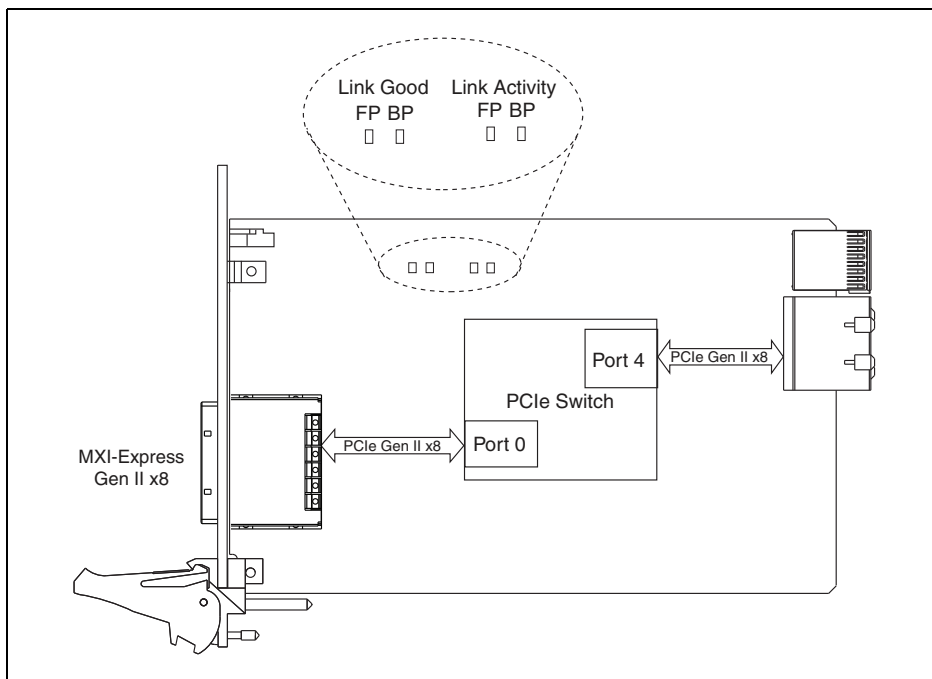
Figure 2-4. NI PXIe-8384 (153100x-01L) Onboard LED Locations
