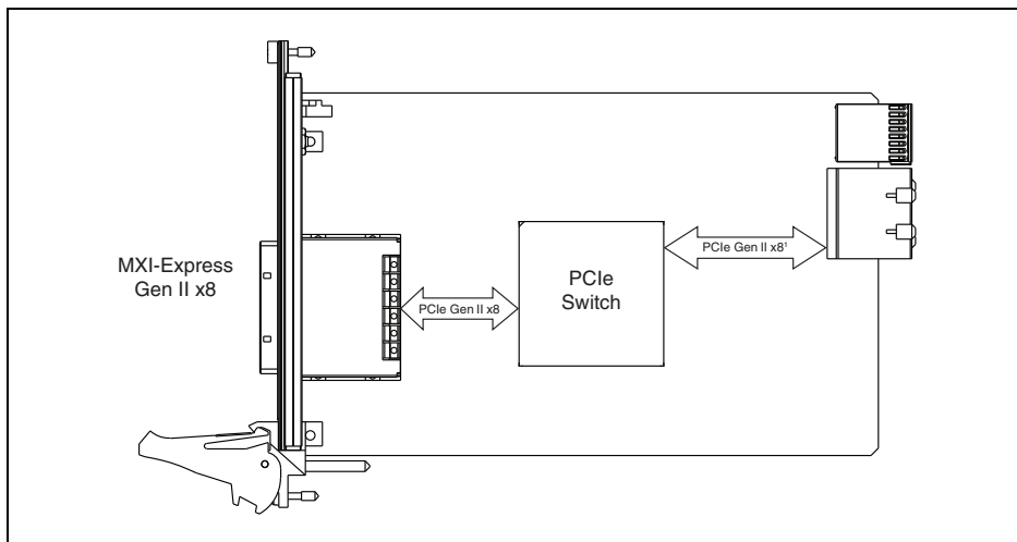
Figure 1-3. NI PXIe-8384 (153100x-01L) Block Diagram 1
