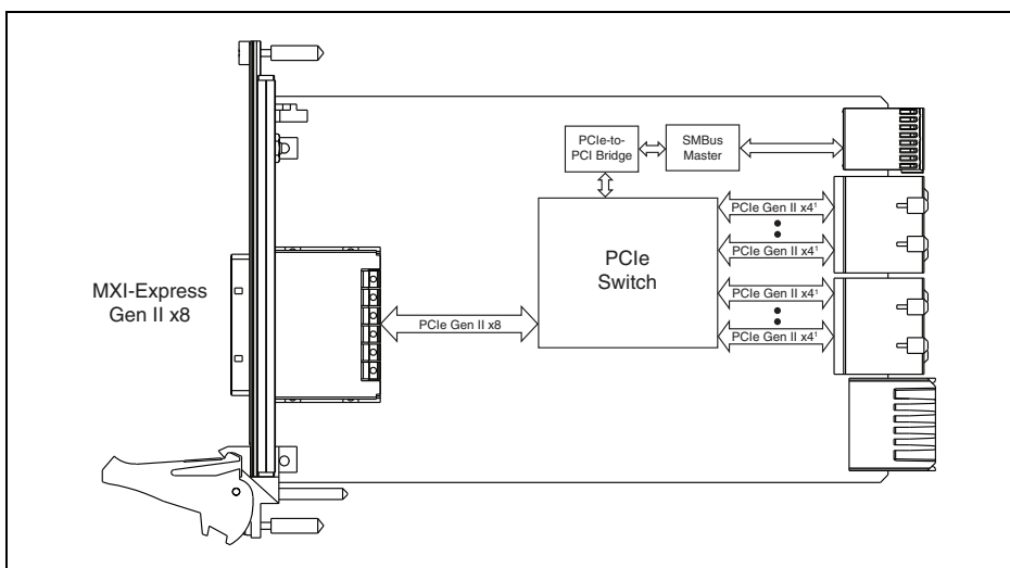
Figure 1-2. NI PXIe-8381 (153097x-01L) Block Diagram 1
