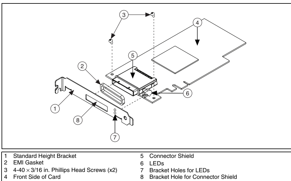
Figure 2-2. Removing the Standard Bracket from the NI PCIe-8381
