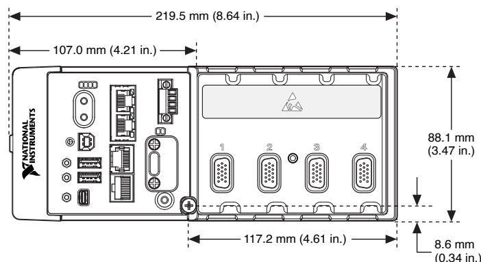
Figure 5. cRIO-9030 Front Dimensions
