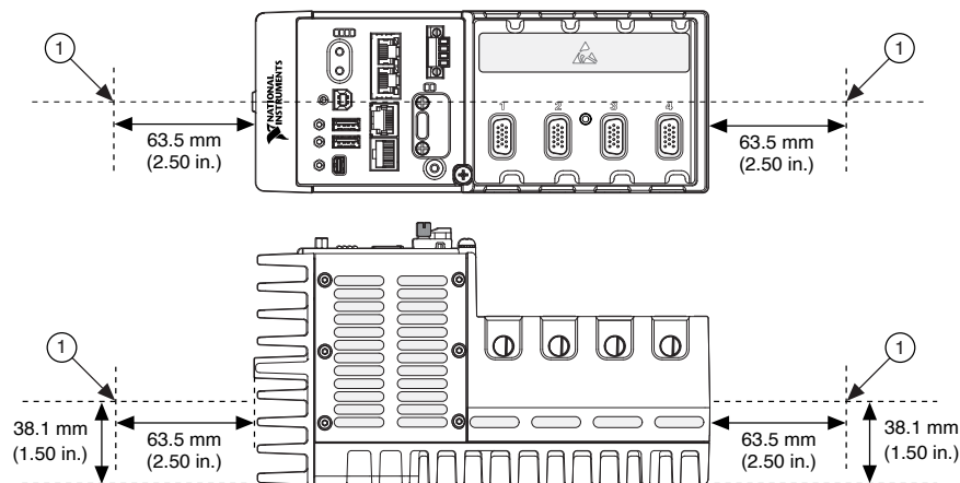
Figure 9. cRIO-9030 Ambient Temperature Location
