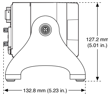
Figure 13. cRIO-9030 Desktop Mounting Side Dimensions
