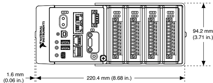
Figure 3. cRIO-9030 Module Immobilization Accessory Dimensions
