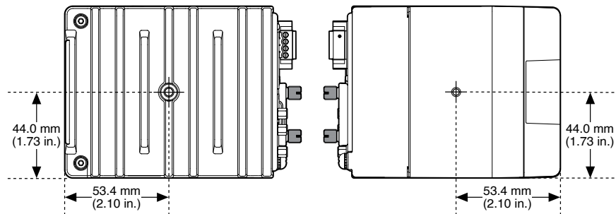
Figure 6. cRIO-9030 Side Dimensions
