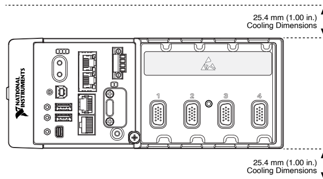
Figure 7. cRIO-9030 Cooling Dimensions
