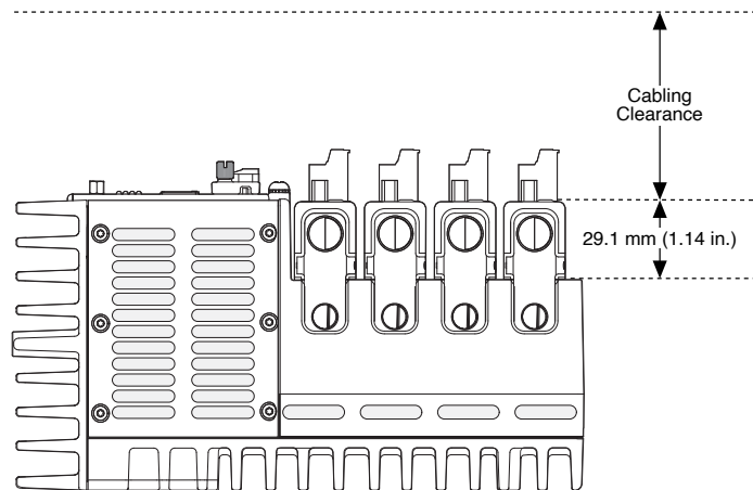
Figure 8. cRIO-9030 Cabling Clearance
