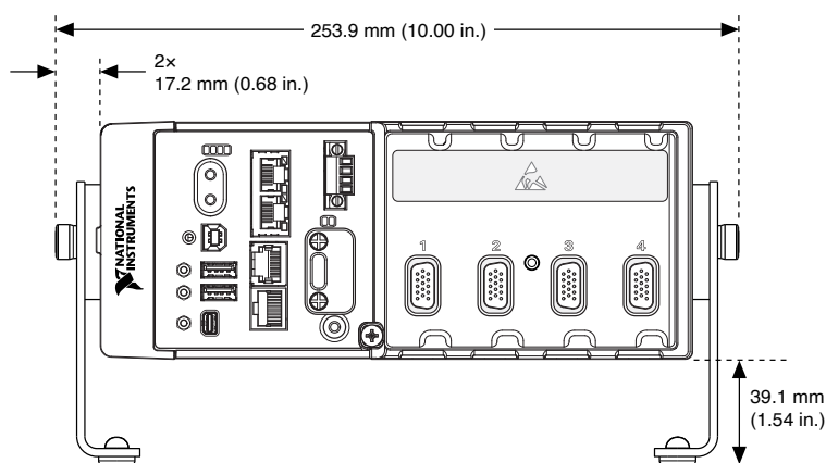
Figure 12. cRIO-9030 Desktop Mounting Front Dimensions
