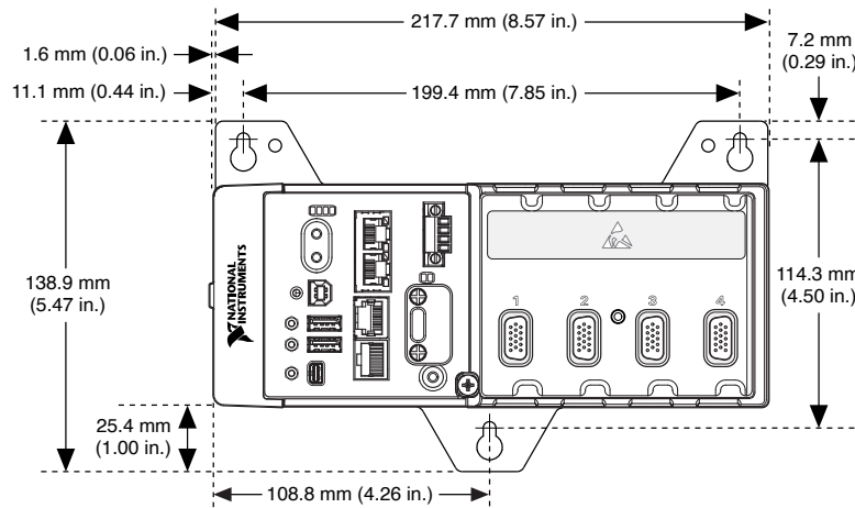
Figure 11. cRIO-9030 Panel Mounting Dimensions
