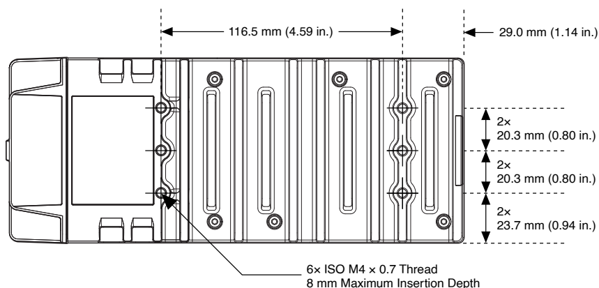
Figure 10. cRIO-9030 Surface Mounting Dimensions
