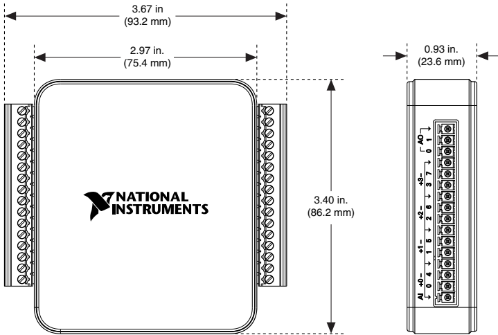
Figure 1. NI USB-6002 Dimensions
